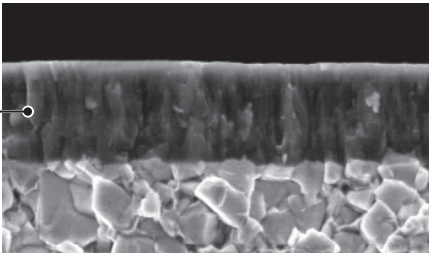
Multi-layer Accumulated Al-Ti-Cr-N Based PVD Coating
