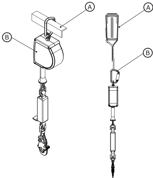
Figure 7 - Connecting to Anchorage
