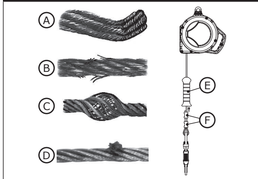
Figure 12 - Wire Rope Lifeline
