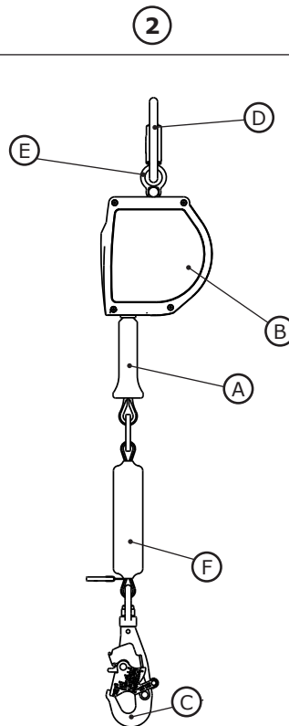
Figure 2 - Components
