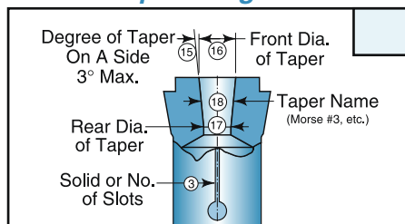
Taper - Regular
