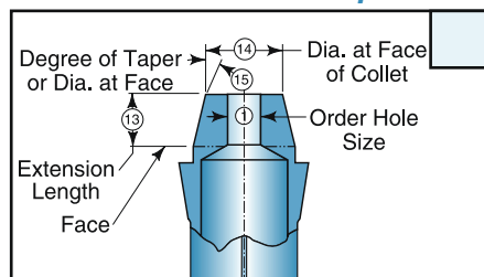
Taper - Reverse
