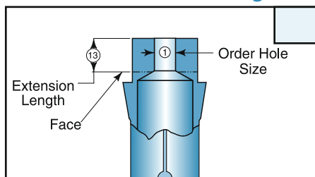
Taper - Regular
