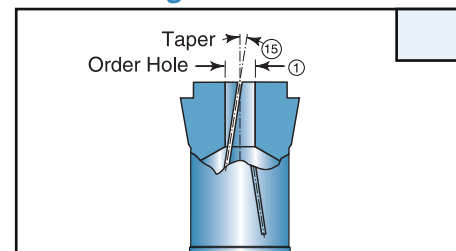
Zig-Zag Slots
